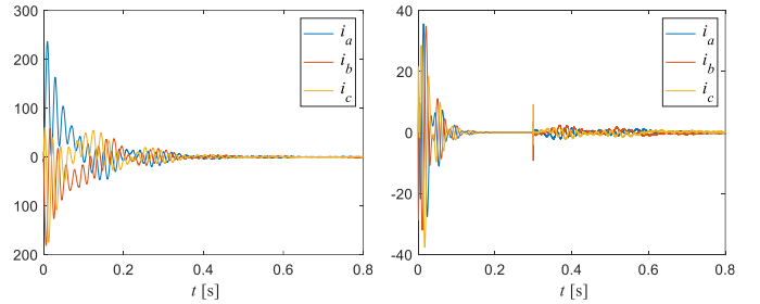
Fig. 7. Waveforms of currents i [A] brought to algorithm without (left) and with synchronization block (right)
