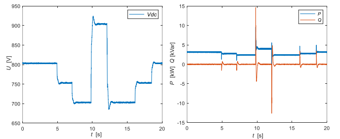
Fig. 11. Wide-range changes in DC voltage (left), active and reactive power during DC reference variation test (right)
