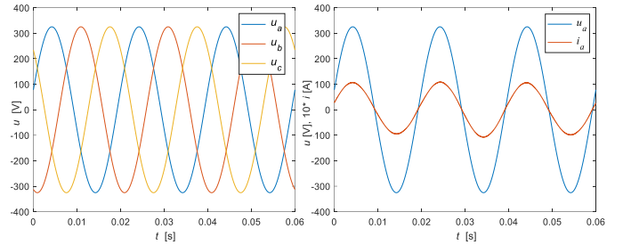
Fig. 10. Grid voltages (left), phase a current and voltage (right)
