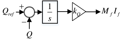
Fig. 5. Structure of reactive power controller
